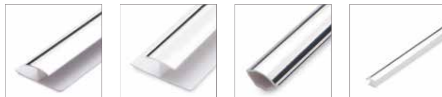
H Trim Chrome 8mm x 2.7m (4010060437) H Trim Chrome 10mm x 2.7m (4010060445) Quadrant Chrome 15mm x 2.7m (4010060475) Chrome Infill Strip 8mm x 2.7m (4010060465)
